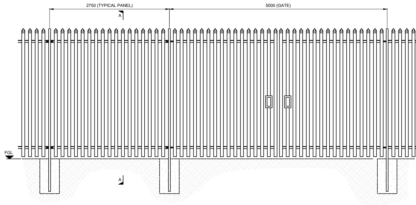
TYPICAL PALISADE FENCE DETAIL
