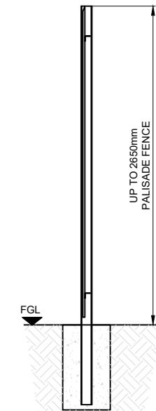
TYPICAL SECTION A-A
